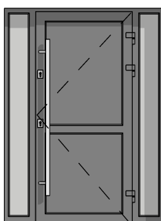
PCV ENTRANCE DOOR TYPE 5 + 2X_NB
