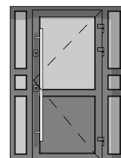
PCV ENTRANCE DOOR TYPE 6B + 2X_NB
