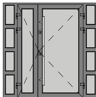
2X_PCV ENTRANCE DOOR TYPE 2C + 2X_NB
