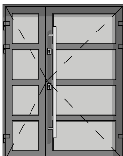
PCV ENTRANCE DOOR TYPE 28A_2X_ASYMETRIC
