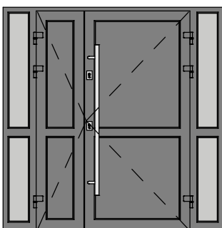
2X_PCV ENTRANCE DOOR TYPE 5A + 2X_NB
