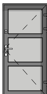
PCV ENTRANCE DOOR TYPE 26
