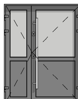
PCV ENTRANCE DOOR TYPE 6_2X_ASYMETRIC
