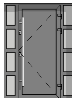
PCV ENTRANCE DOOR TYPE 1C + 2X_NB
