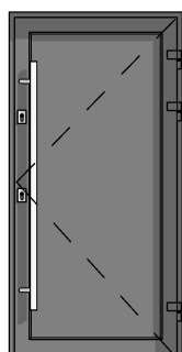
PCV ENTRANCE DOOR TYPE 1
